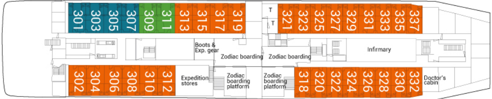
Deck 3
